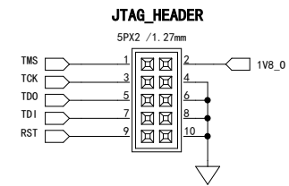
JTAG_HEADER
